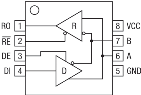
WT714H and WT718H Pinout (TopView)
