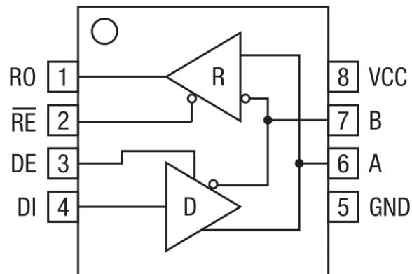
WT714H and WT718H
