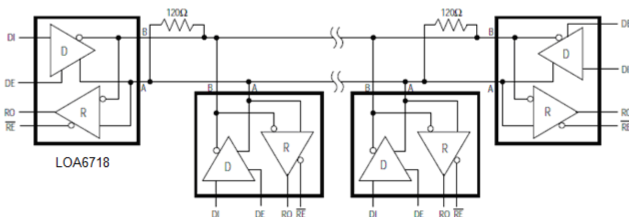
Figure 10. LOA6718 Typical RS-485 Network
