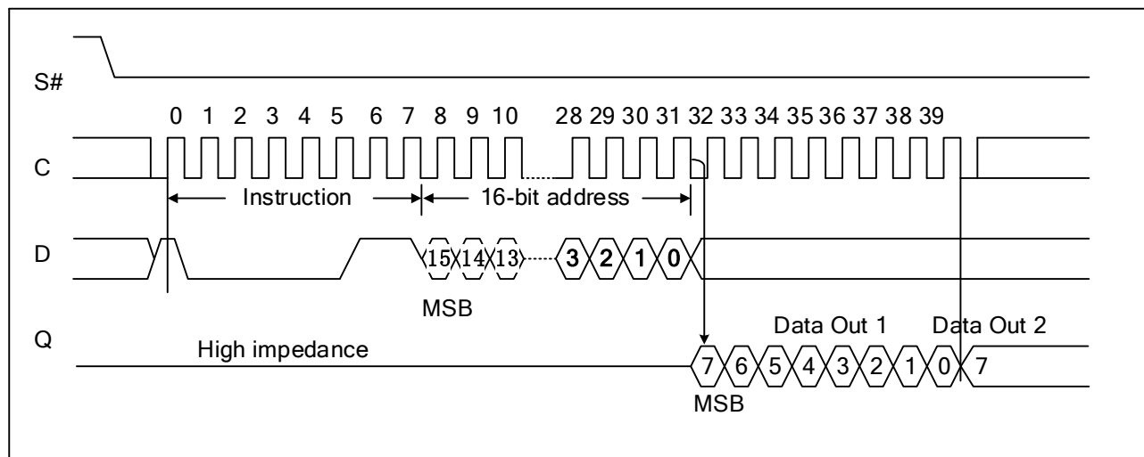
Figure 6-11. Read Identification Page sequence
