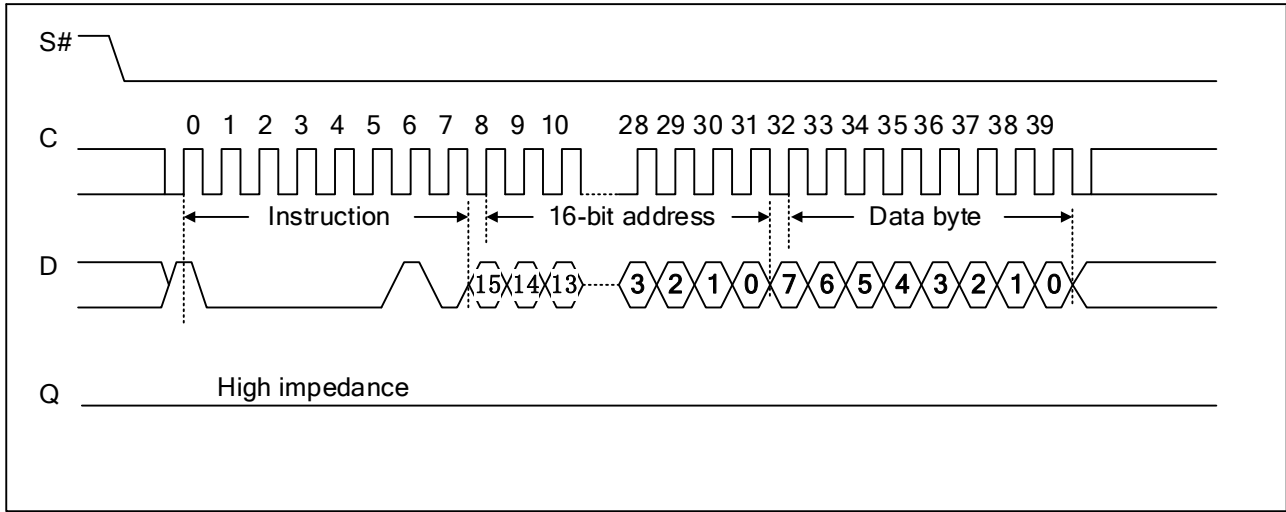
Figure 6-12. Write Identification Page sequence
