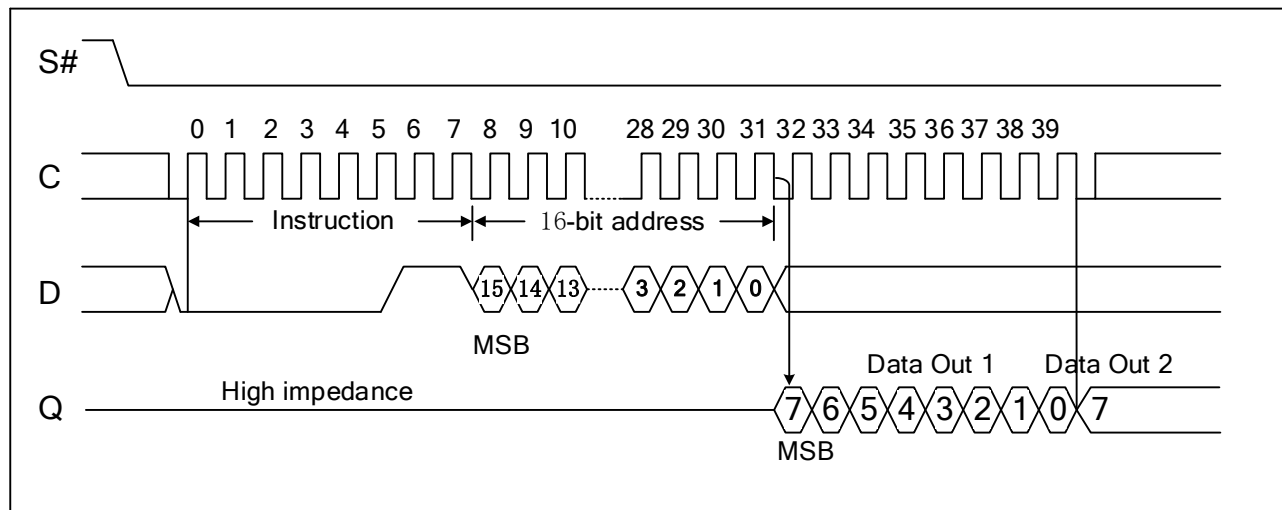
Figure 6-8. Read from Memory Array (READ) sequence
